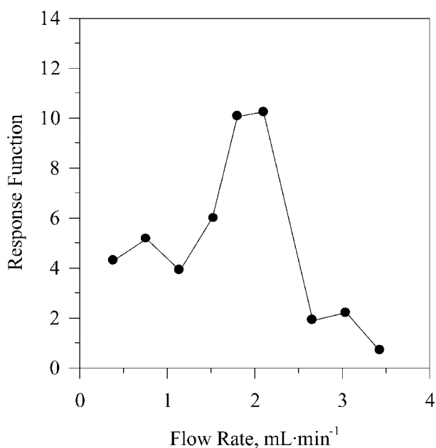
Figure 2. Effect of flow rate on the Response Function. Sample volume: 566 µL; reaction coil: 3 m; reagent dilution: n = 10.
